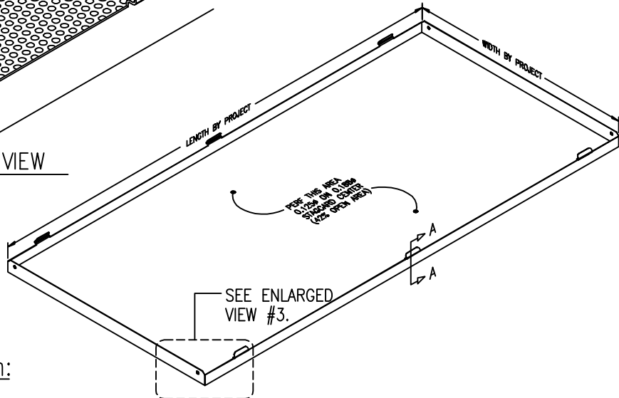
② TYP. SCREEN - ISO VIEW SCALE: NONE
