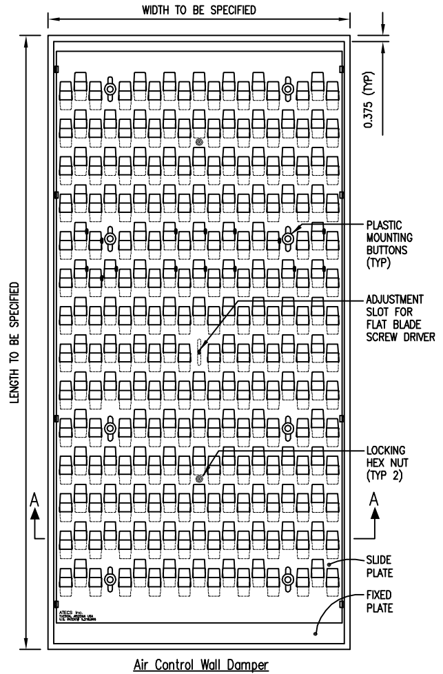
Air Control Wall Damper
