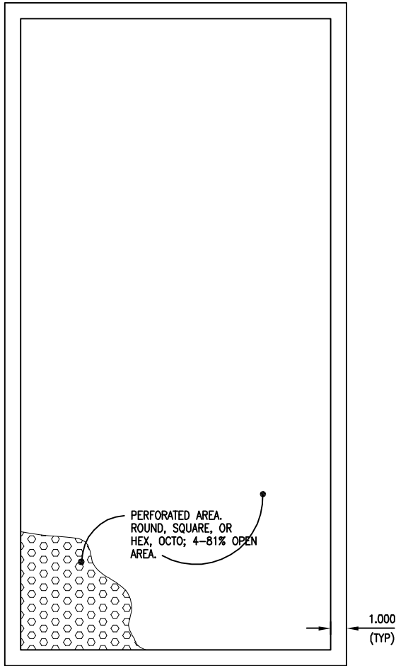
① PERFORATED RETURN AIR GRILLE
