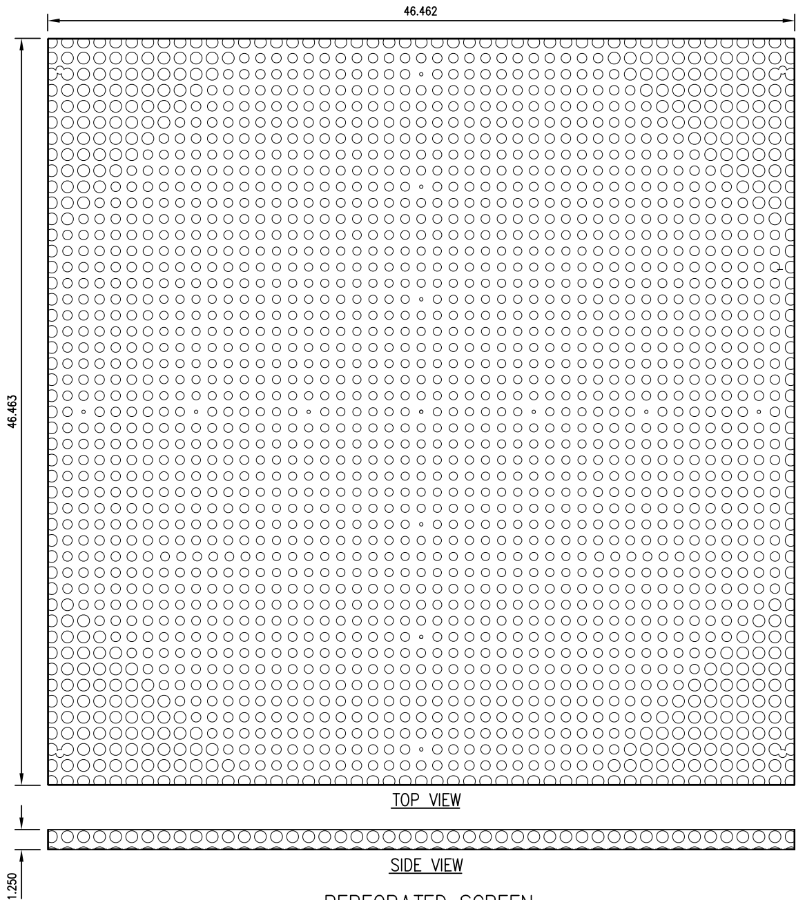
① PERFORATED SCREEN
