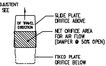
2 DAMPER ADJUSTMENT ASSEMBLY
