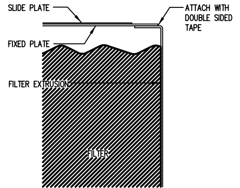
5 ENLARGED DETAIL
