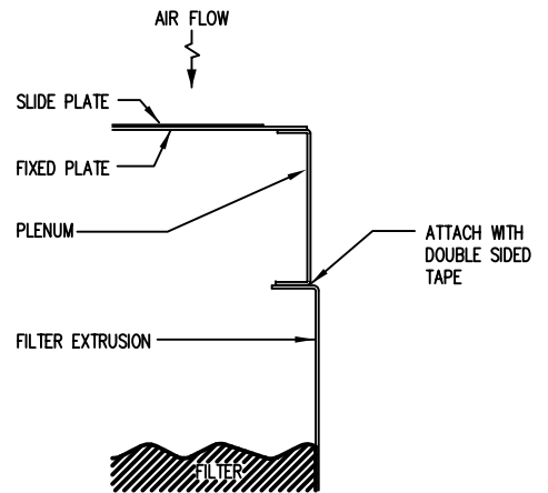
5 ENLARGED DETAIL
