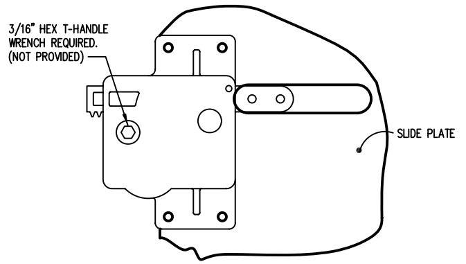
2 DAMPER ADJUSTMENT ASSEMBLY
