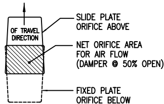
3 ORIFICE DETAIL
